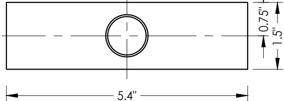
9 TUBE ANCHOR
